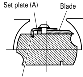
Fig. 10 (Correct installation)
