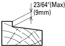
Fig. 2-D (Tapering)
